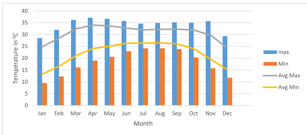
Figure 6.17: Monthly maximum, minimum and average temperature (1987-2017)
