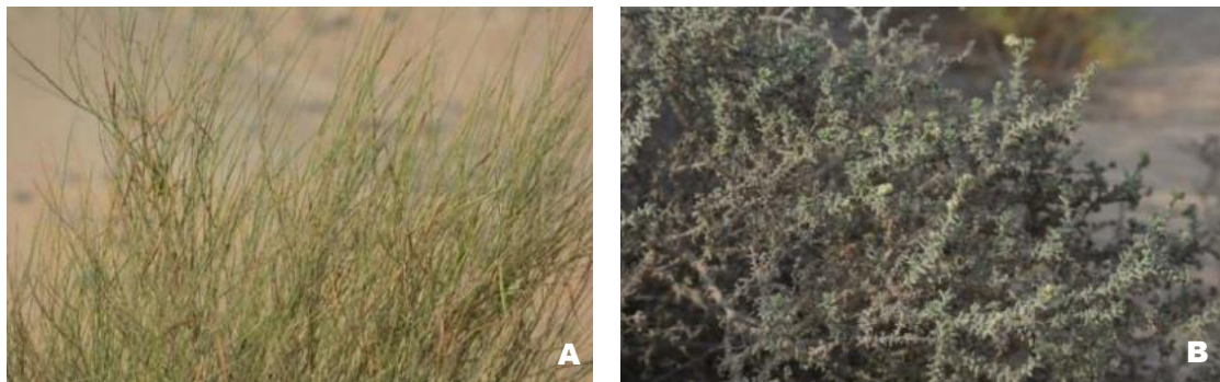
Plate 5-8 Dominant Plant Species at the Project site: (A) Leptadenia pyrotechnica , and (B) H bacciferum
