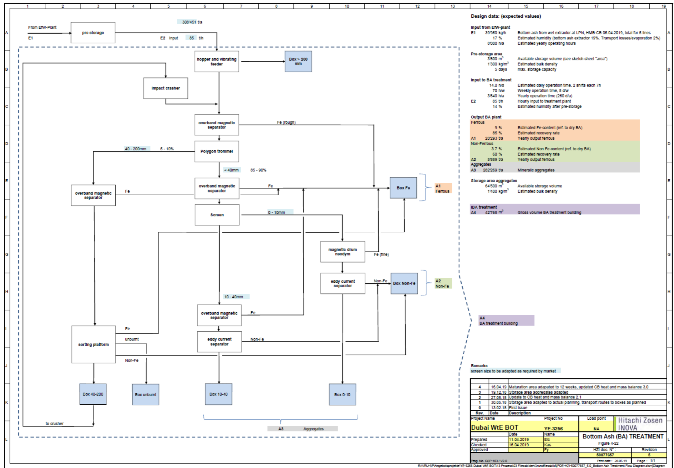
Figure 4-22 Bottom Ash Treatment Flow Diagram
