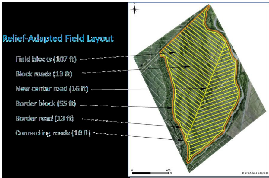
Figure 2.1-3: The field layout is adapted to the relief. The center road follows the watershed and the orientation of the field blocks is approximately parallel to the contour lines.
