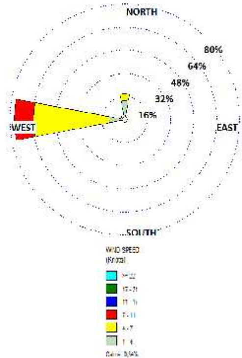
Gambar 2.3. Windrose Bulan November-April
