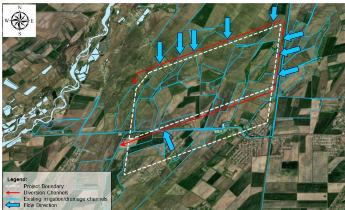
Figure 14: Drainage Diversion Concept
