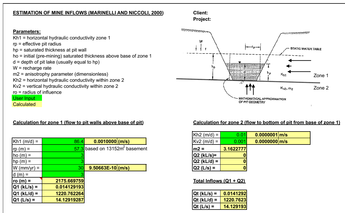
Figure 16: Inflow estimation working 1 (Marinelli and Niccoli Eqn)
