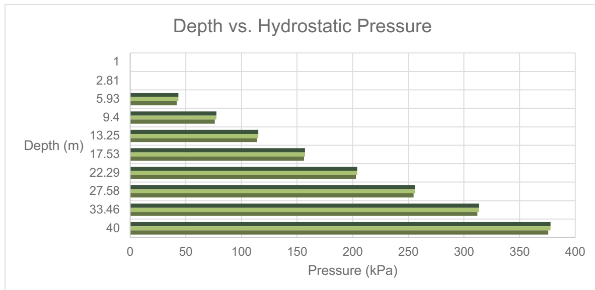
Figure 8: Depth Vs Hydrostatic Pressure (Haskoning, 2025)
