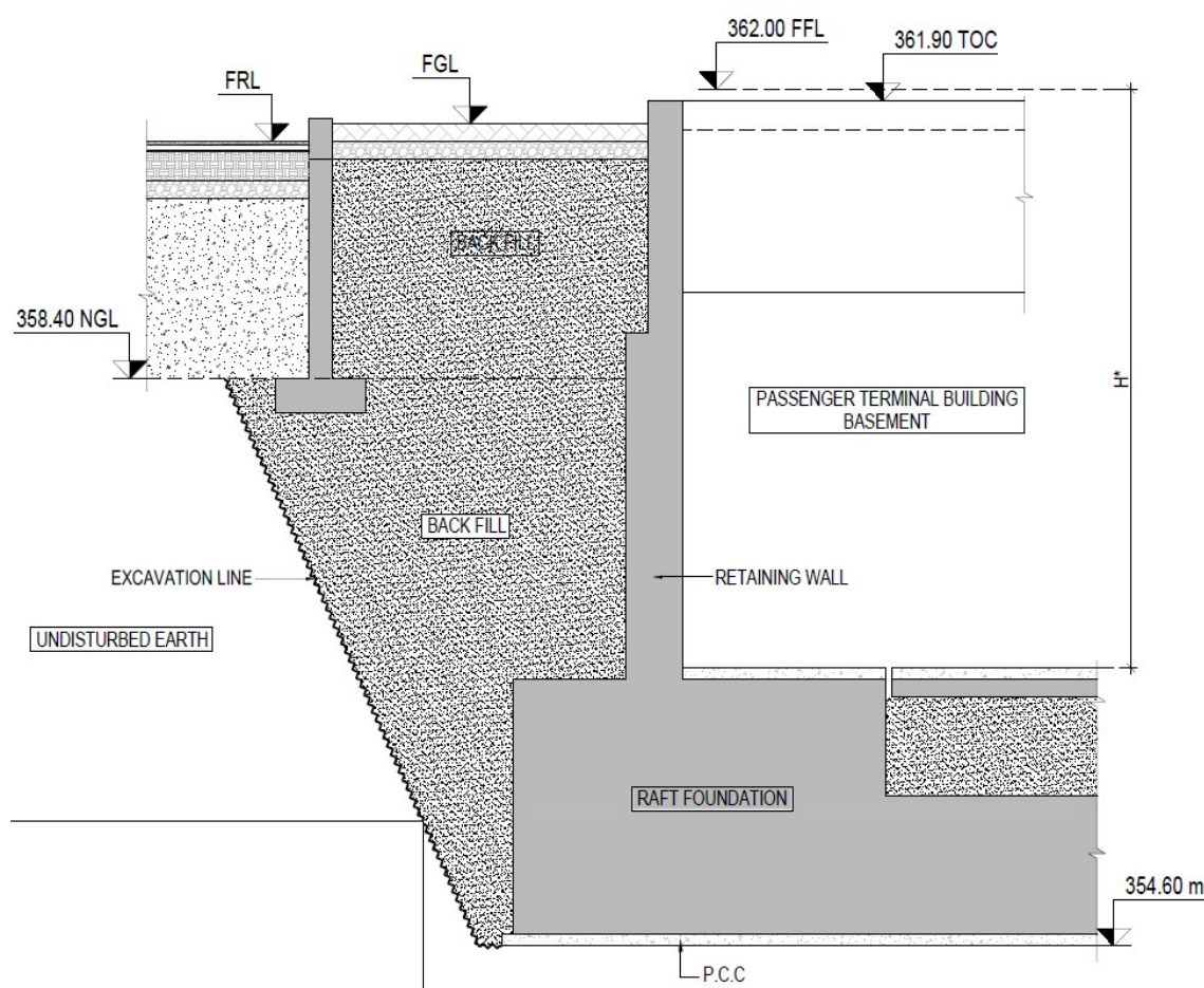
Figure 13 Cross section of excavation chamber for Passenger Terminal Basement
