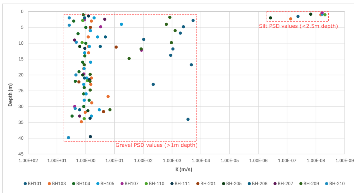
Figure 7: Kozeny-Carman analysis
