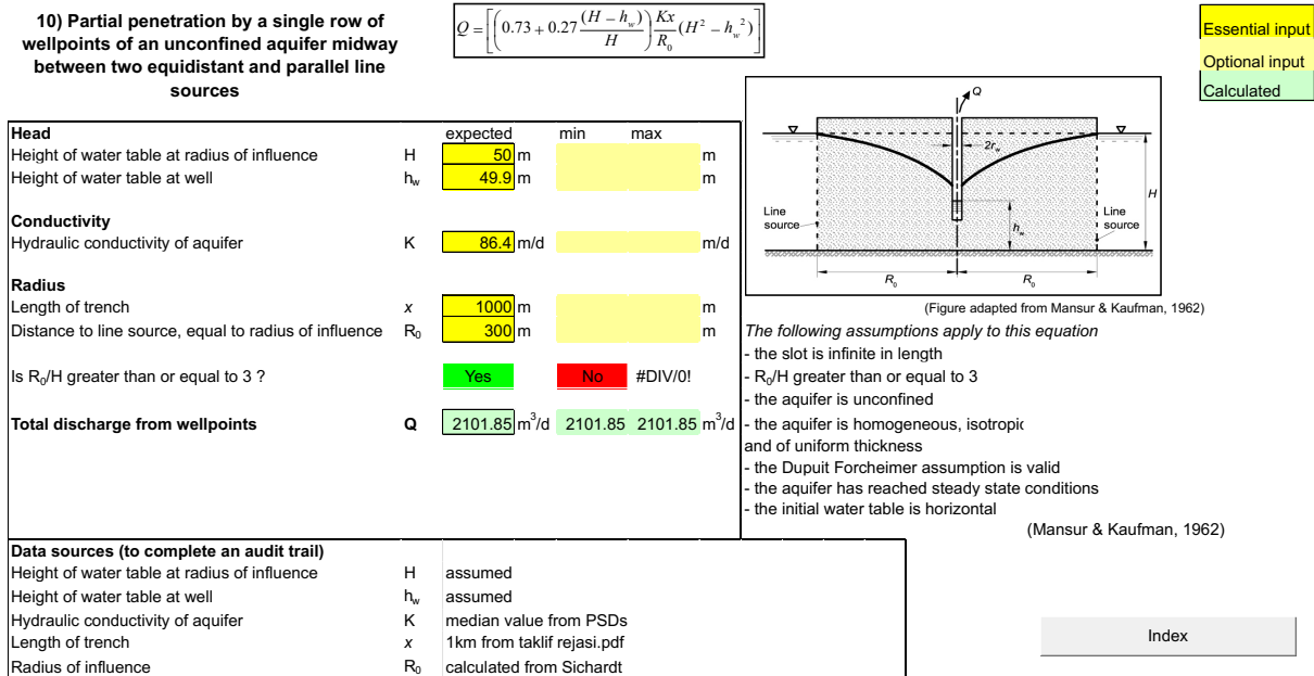
Figure 17: Inflow estimation working 2
