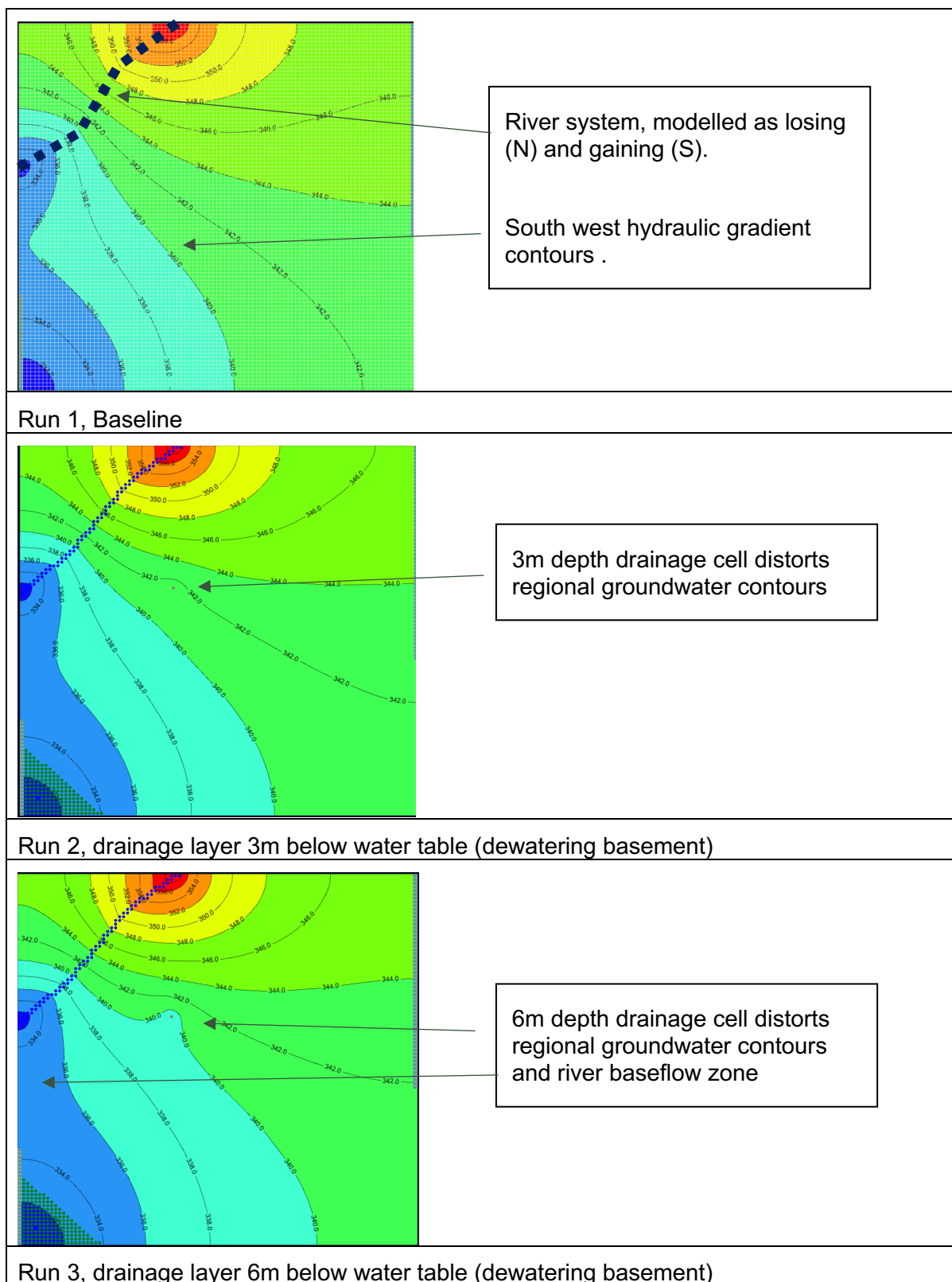
Figure 20: Example Water Table Results, Numerical Modelling
