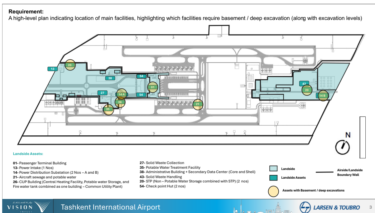
Figure 12: Airport Terminal main Facilities with sub-water table excavations
