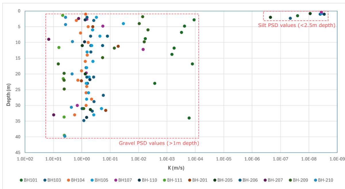
Figure 6: Hazen analysis
