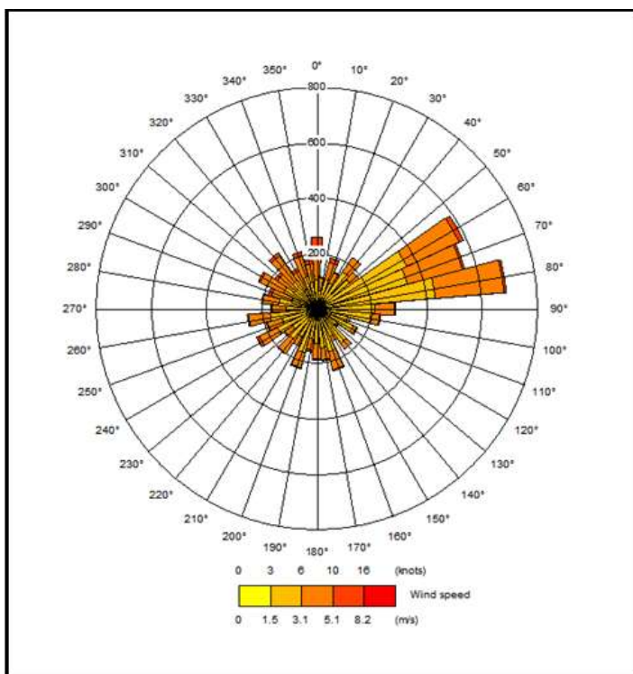
Figure 3.5: Wind rose for Tashkent International Airport (2024)
